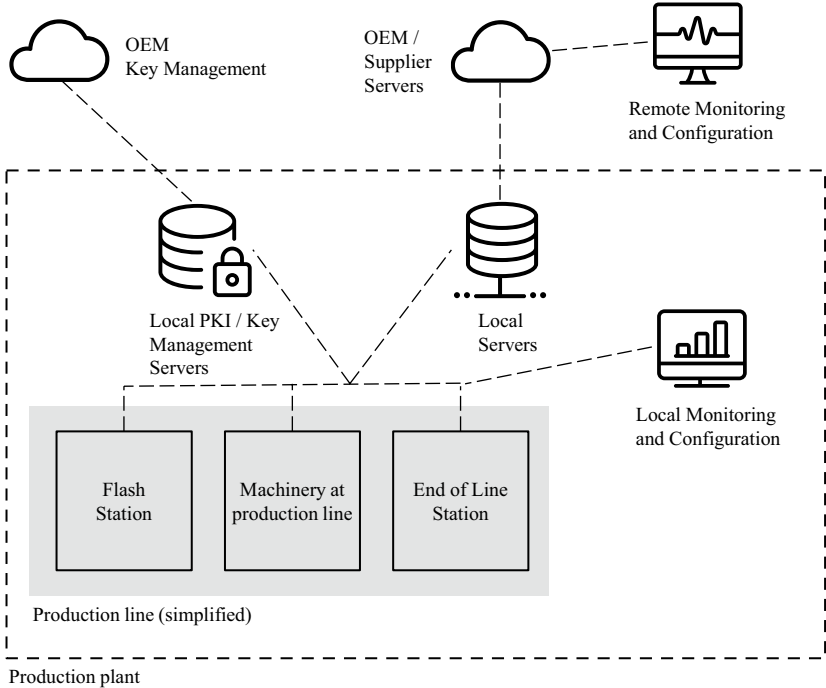
Fig. 5.5 Production plant including a production line and diverse back-end communication systems
